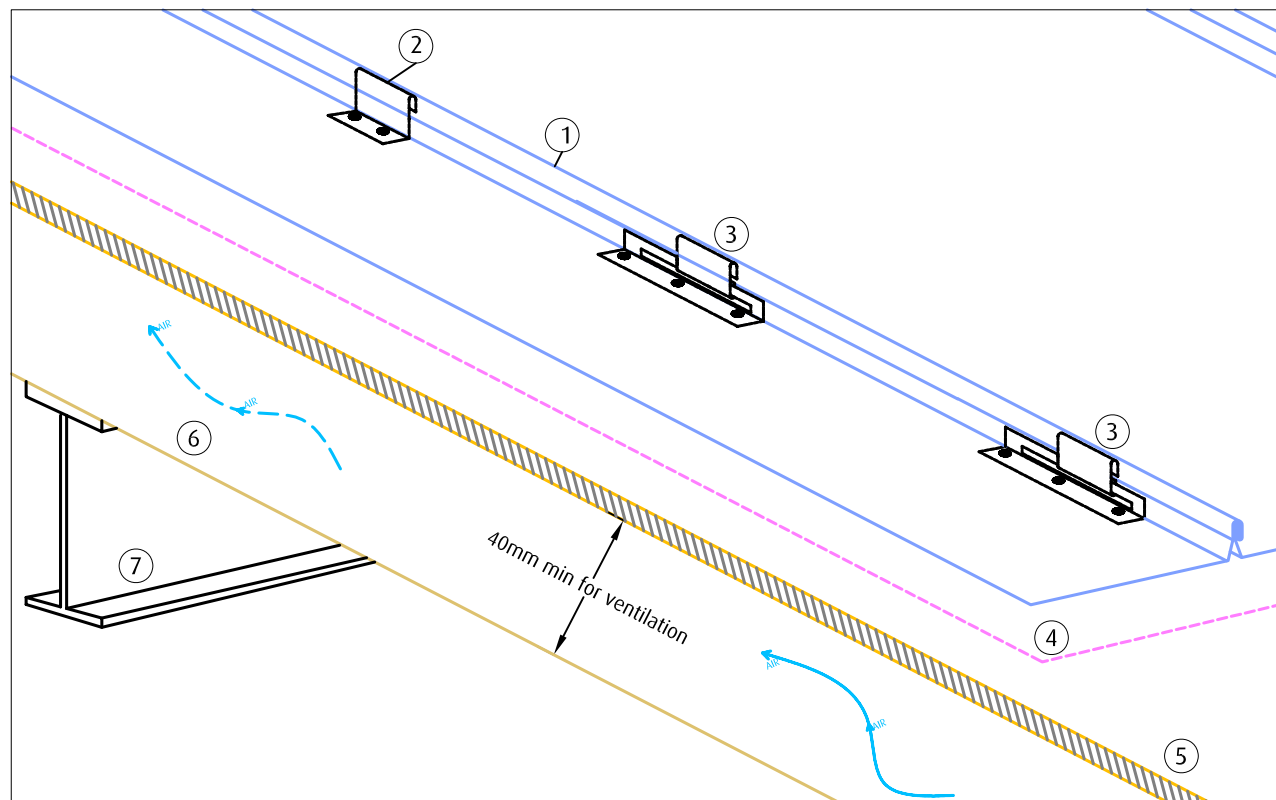
fixing clips
