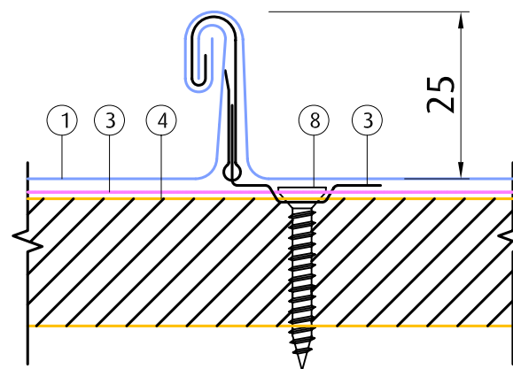
seam joint
