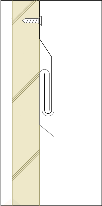
Recessed Joint
