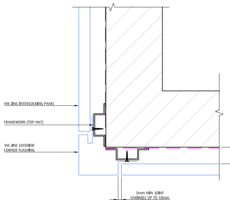
CORNER FLASHING
